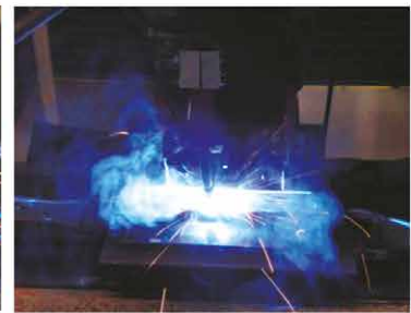
TAWERS MTS-CO 2 (%100 CO 2 )
